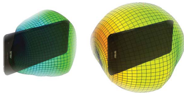
Single Antenna
