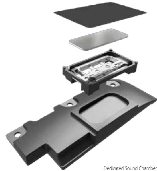
Dedicated Sound Chamber Designed for Five Magnet Speaker
