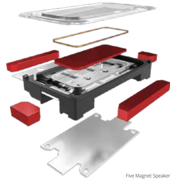
Five Magnet Speaker
